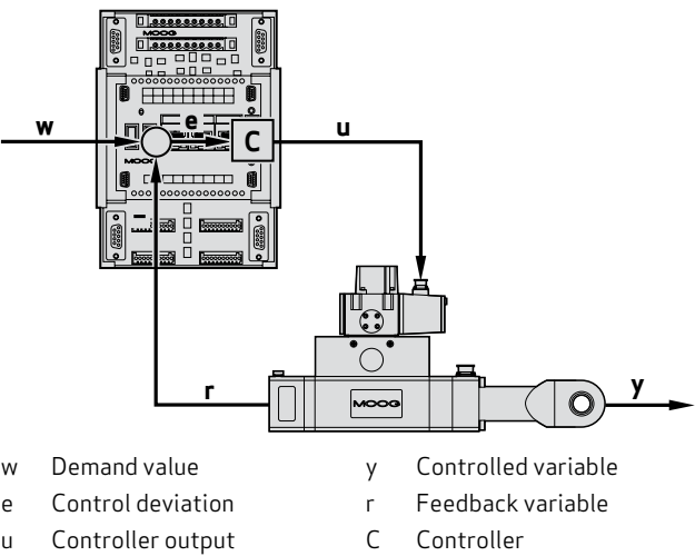
Control loop consisting of controller and valve-actuated cylinder with position transducer
