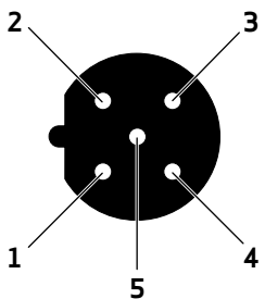
View on Profibus-DP connector X4
