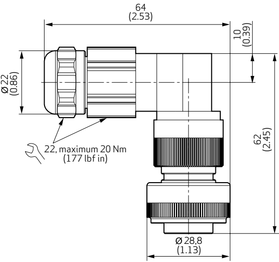
Mating connector, elbow 6-pole + PE
