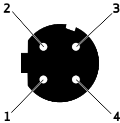
View on EtherCAT connector X4
