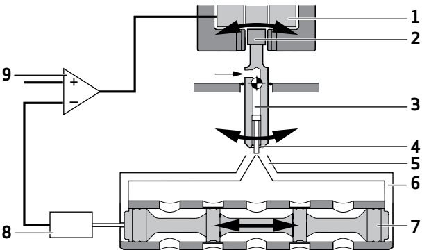
Principle of operation of the ServoJet® Pilot Stage
