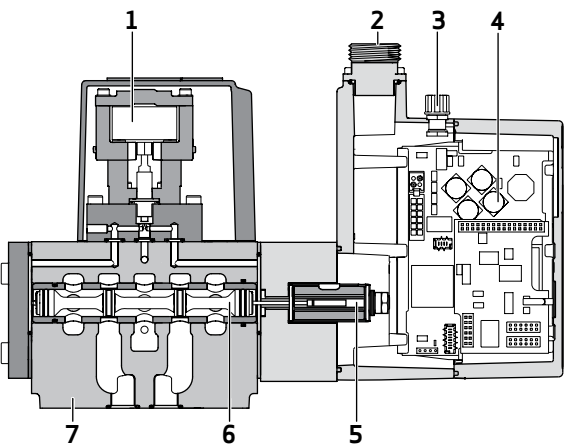
Cutaway view, 2-stage servovalve
