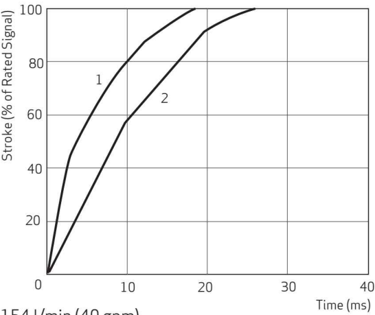
154 l/min (40 gpm) Plot 1 @ 210 bar (3,000 psi) Plot 2 @ 70 bar (1,000 psi)
