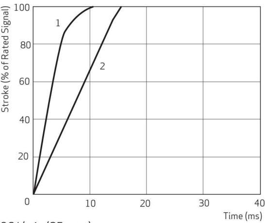
96 l/min (25 gpm) Plot 1 @ 210 bar (3,000 psi) Plot 2 @ 70 bar (1,000 psi)
